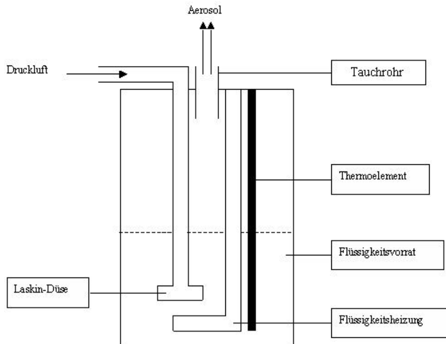
Fig. 2: Schematic diagram of the PLG 2000 H aerosol generator Startup The liquid to be dispersed is simply filled in the reservoir. The nozzle system developed by Palas® is immersed in the liquid. This nozzle system is based on the Laskin principle and guarantees extremely precise dosing constancy with uniform particle size. The mass flow is adjusted using the volume flow through the nozzle. The volume flow is controlled by a pressure regulator and a manometer on the device.
